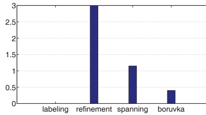
Fig. 13 Percentage of out-of-domain elements running with 8 cores and 16 bottom-level subdomains
