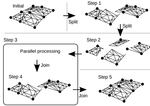
Fig. 2 Structure of the domain-based parallelization of irregular algorithms
