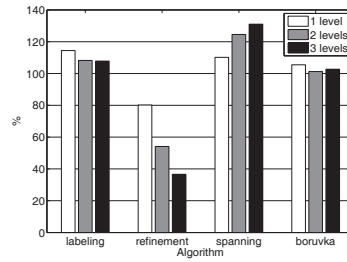
Fig. 12 Speedup with respect to no over-decomposition in runs with 8 cores
