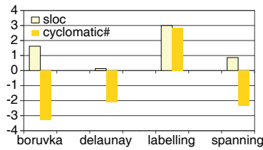
Fig. 10 Relative values of the SLOCs and the cyclomatic number of the parallelized version with respect to the sequential one
