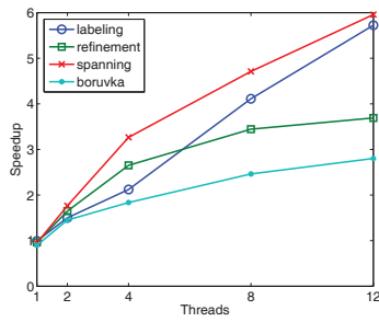
Fig. 11 Speedups with respect to optimized serial versions
